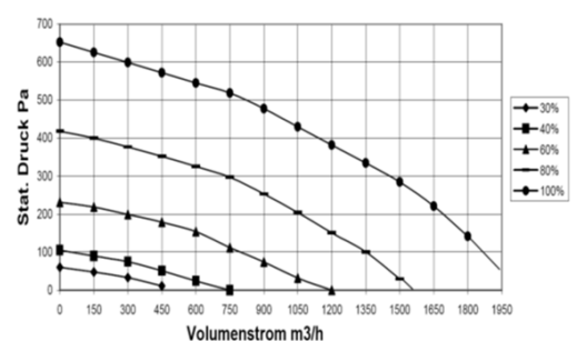
Volumenstrom EuroAir Klimabox 1600
