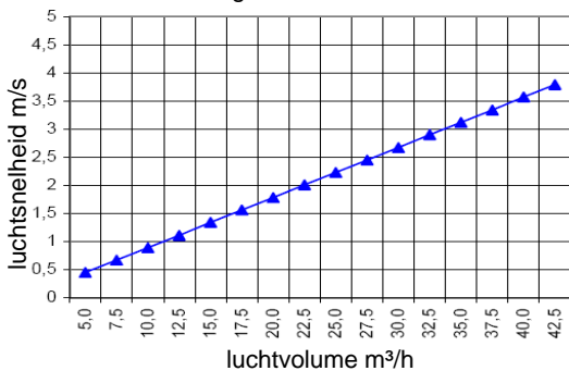
Swenslang volumetabel DIA 75 mm
