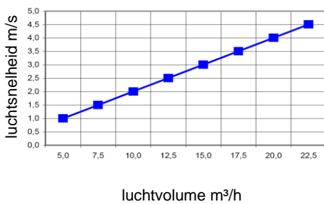
Swenslang volumetabel DIA 50 mm
