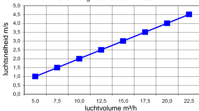
Swenslang volumetabel DIA 50 mm
