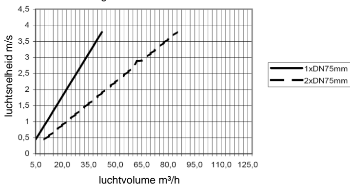
Swenslang volumetabel DIA 75 mm
